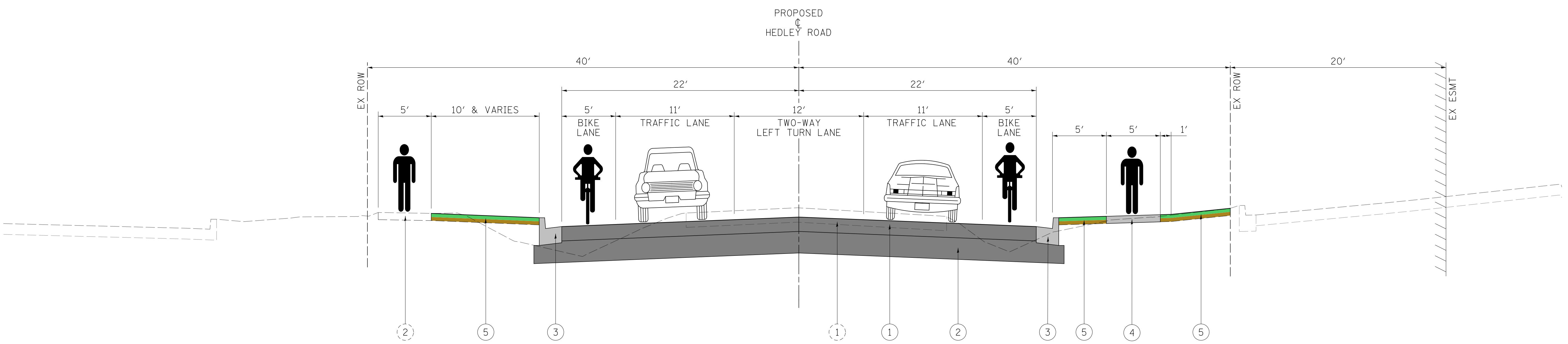
PROPOSED TYPICAL SECTION B-B
