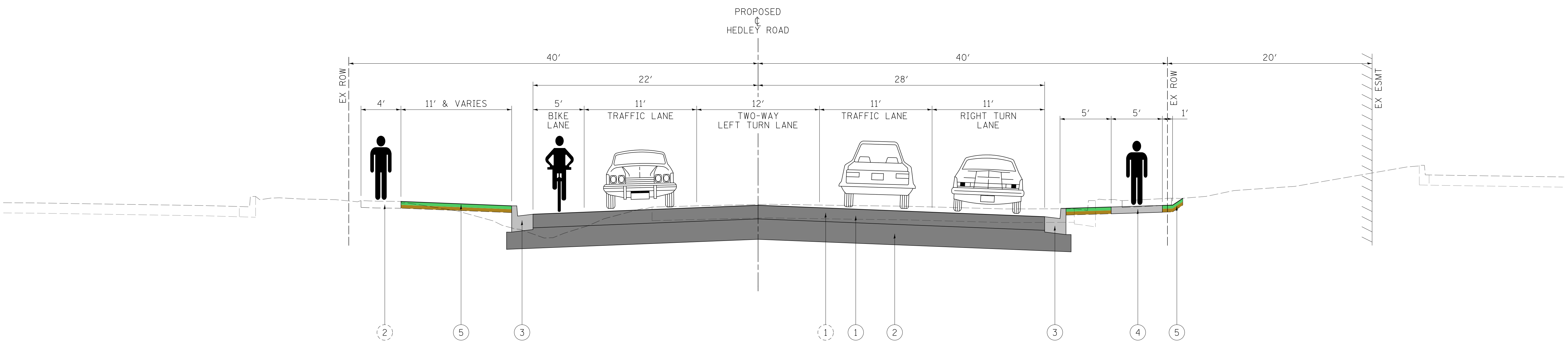
PROPOSED TYPICAL SECTION C-C (SIGNALIZED ALTERNATIVE)
