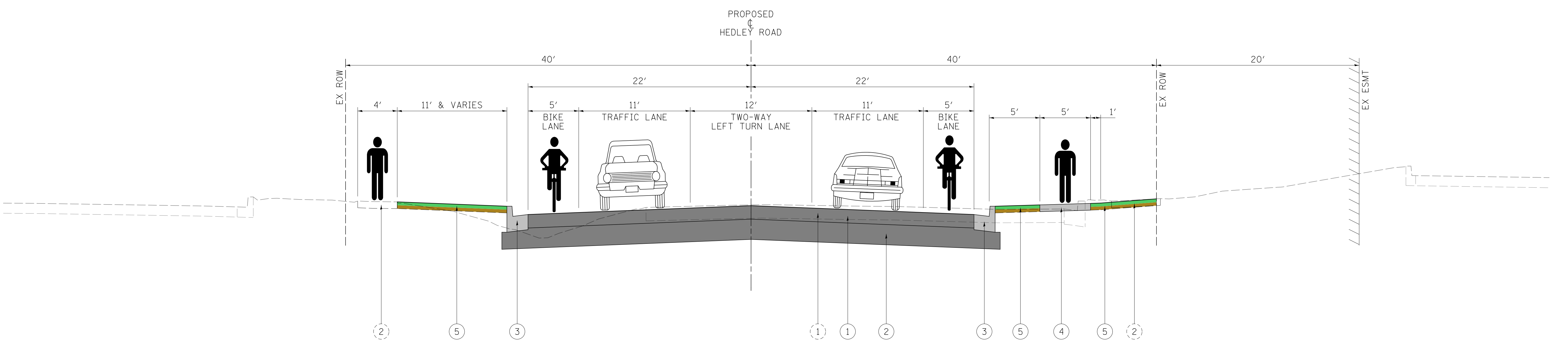
PROPOSED TYPICAL SECTION D-D (3/4 ACCESS ALTERNATIVE)
