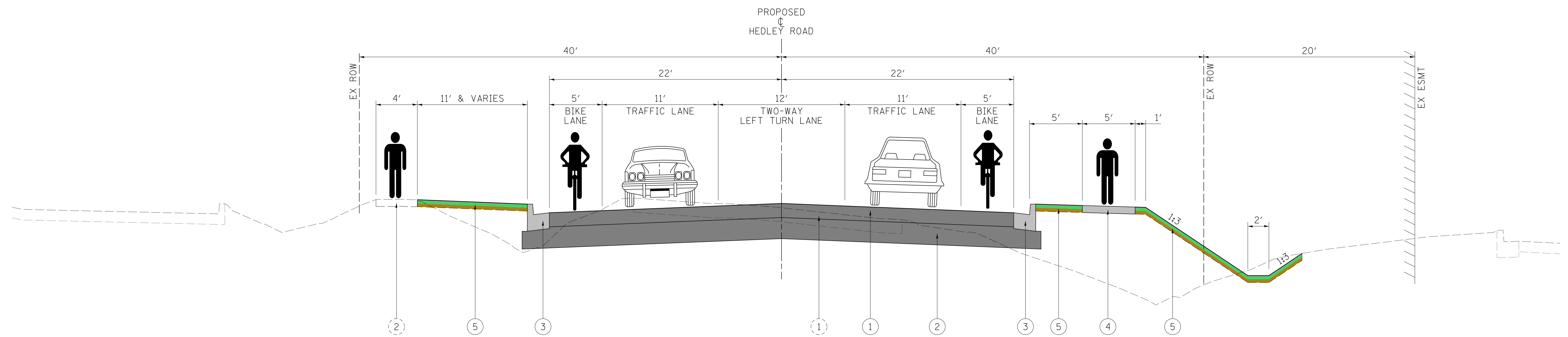
PROPOSED TYPICAL SECTION A-A
