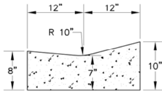
COS - VALLEY TYPE GUTTER
