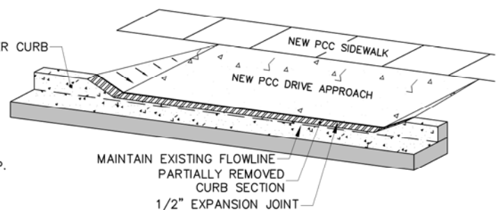
TYPICAL TAPERED APPROACH TRANSITION
