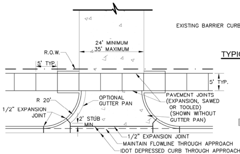
TYPICAL COMMERCIAL DRIVE APPROACH WITH RADIUS
