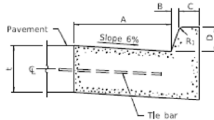
BARRIER CURB
