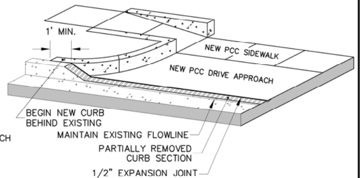
TYPICAL RADIUS APPROACH CURB TRANSITION - CASE 2
