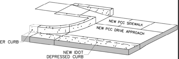
TYPICAL RADIUS APPROACH CURB TRANSITION - CASE 1
