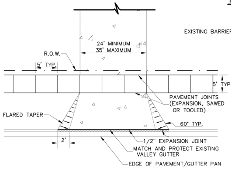
TYPICAL COMMERCIAL DRIVE APPROACH WITH TAPER
