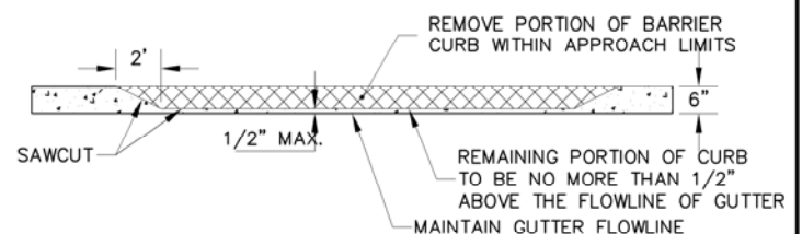
TYPICAL CURB SAWCUTTING THRU APPROACH
